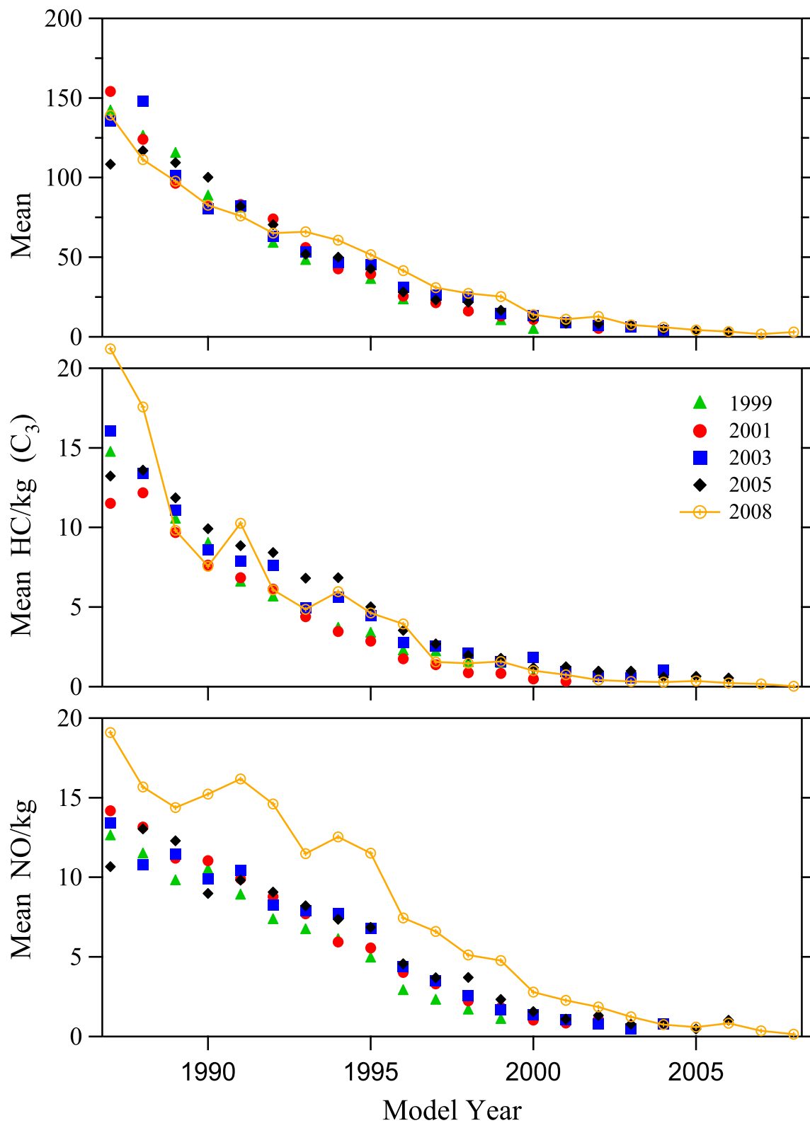
Figure 21. Mean vehicle emissions illustrated as a function of model year. HC data have been offset adjusted as described in the text.
