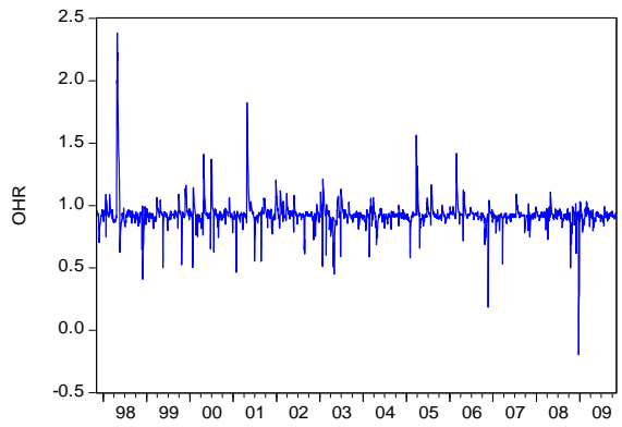
DCC:WTISP_WTIFU
