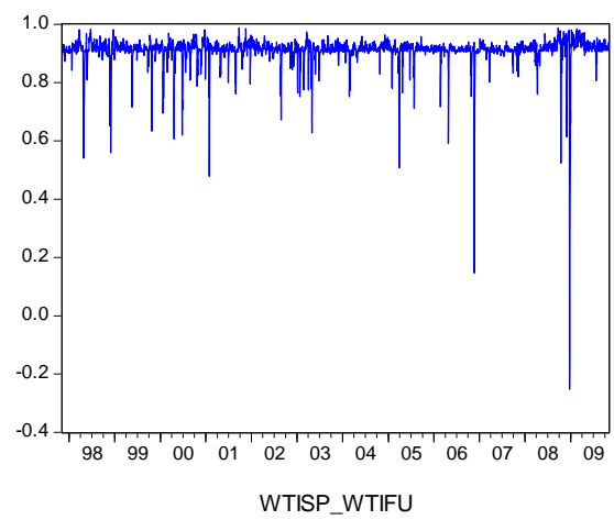
Figure 4. DCC Estimates
