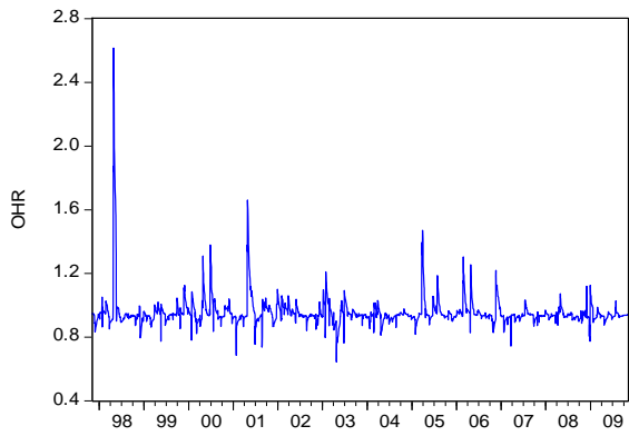
CCC:WTISP_WTIFU
