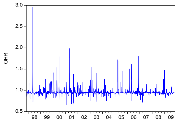
VARMA-GARCH:WTISP_WTIFU
