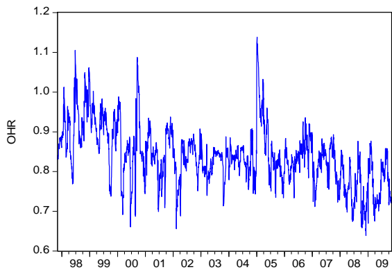
CCC:BRSP_BRFU
