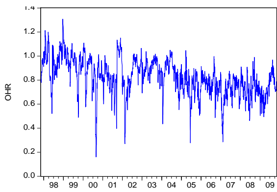
DCC:BRSP_BRFU
