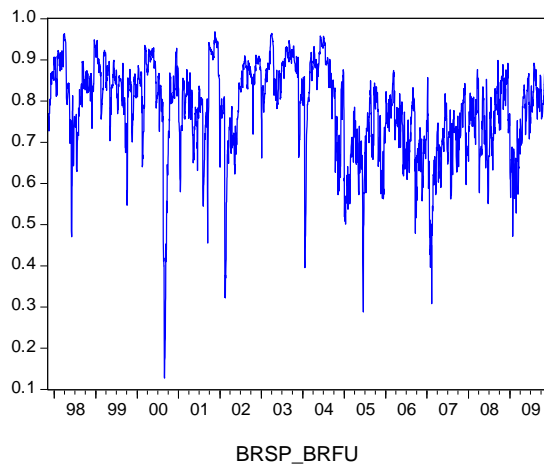
Figure 4. DCC Estimates
