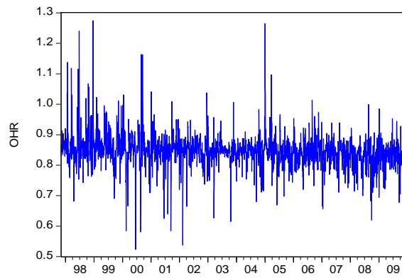
VARMA-GARCH:BRSP_BRFU
